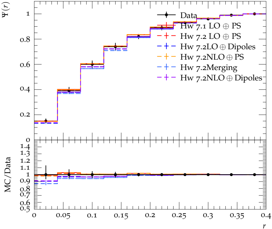
Integrated jet shape for b -jets with 30 \text{ GeV} < p_T < 40 \text{ GeV}
