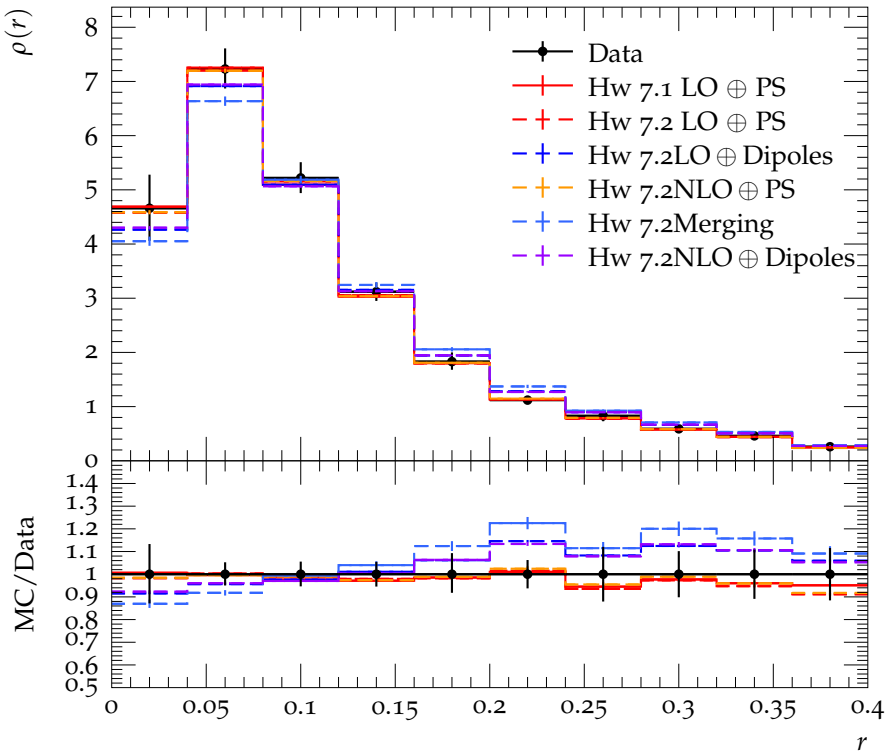
Differential jet shape for b -jets with 40 \text{ GeV} < p_T < 50 \text{ GeV}
