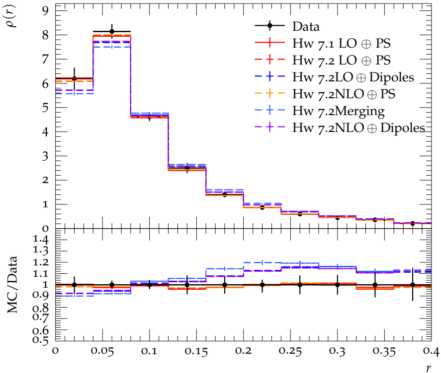
Differential jet shape for b -jets with 50 \text{ GeV} < p_T < 70 \text{ GeV}
