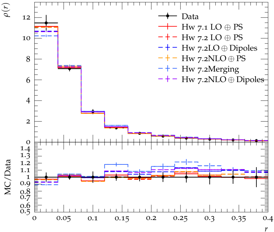
Differential jet shape for b -jets with 100 \text{ GeV} < p_T < 150 \text{ GeV}
