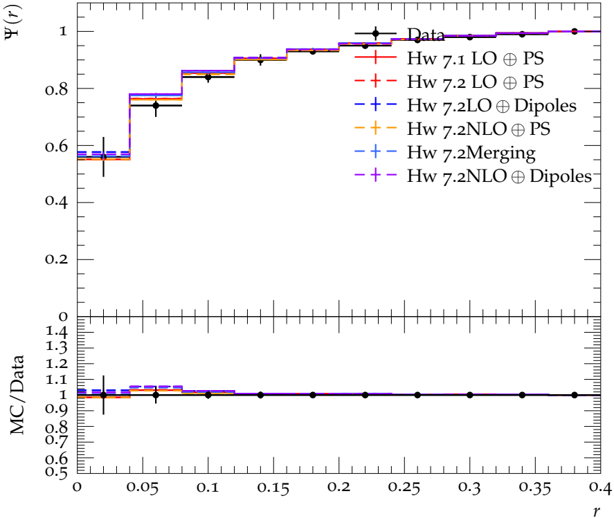
Integrated jet shape for light jets with 100 \text{ GeV} < p_T < 150 \text{ GeV}
