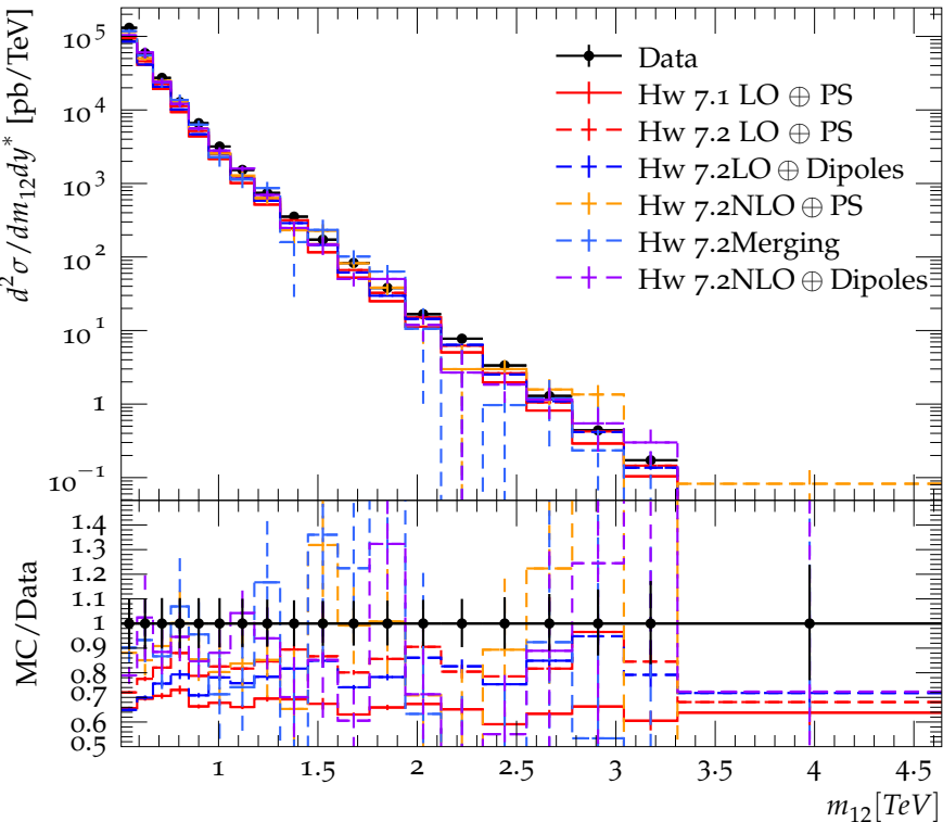
Dijet double-differential cross sections ( 1.0 < y^* < 1.5 ), R=0.4
