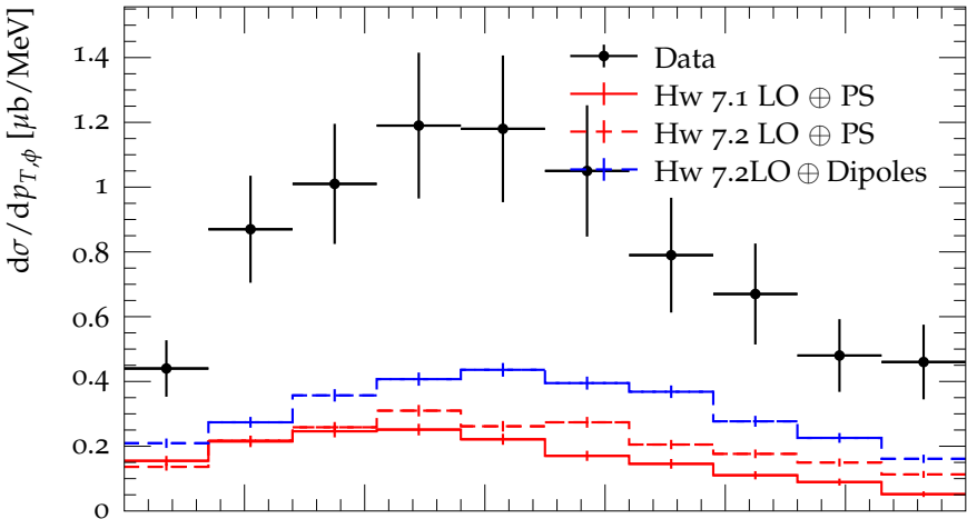
Fiducial \sigma(\phi \rightarrow K^+ K^-) differential in p_{T,\phi}
