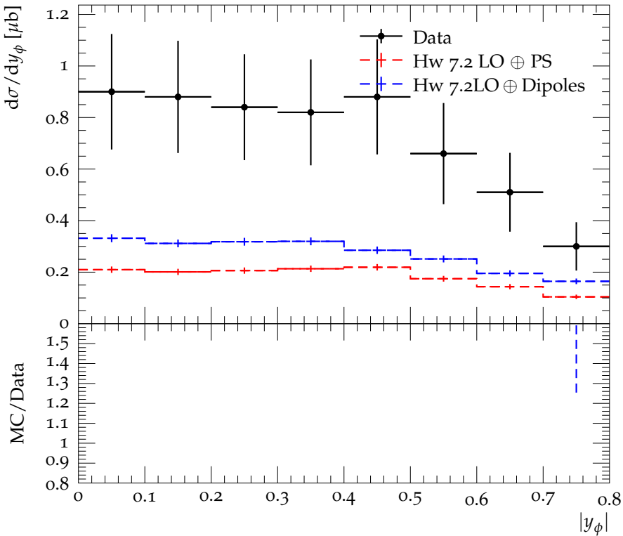
Fiducial \sigma(\phi \rightarrow K^+ K^-) differential in |y_\phi|
