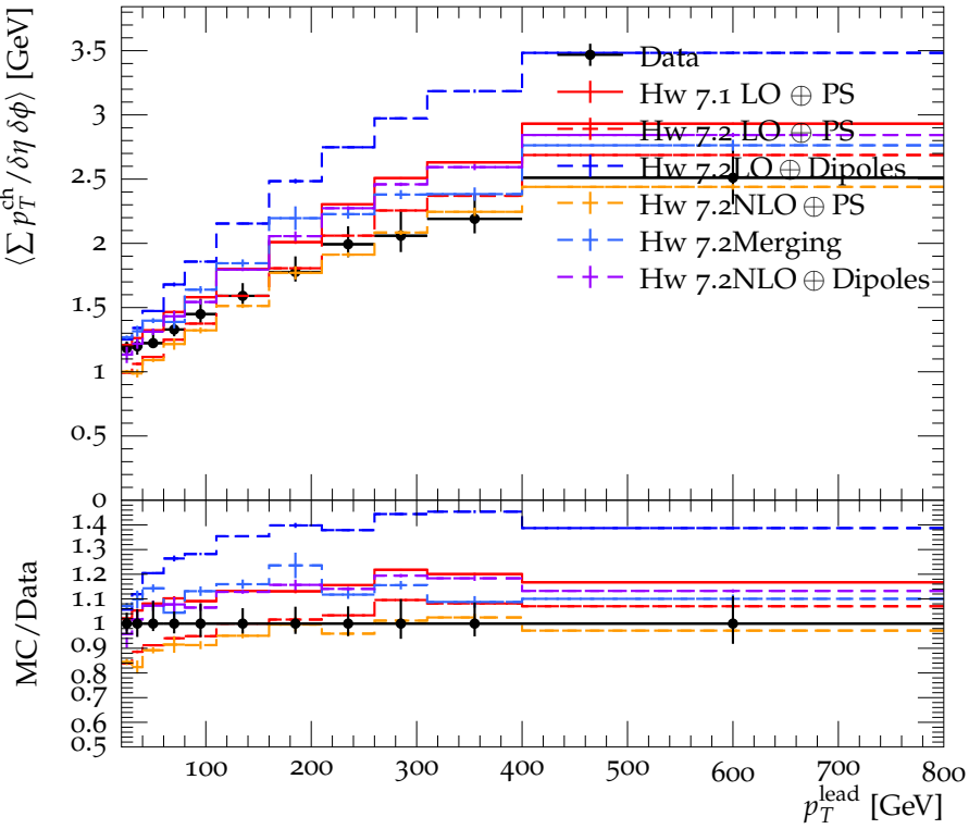
Transverse \langle \sum p_T^{\text{ch}} / \delta\eta \delta\phi \rangle vs. p_T^{\text{lead}} in |\eta| < 2.5 in incl jet events
