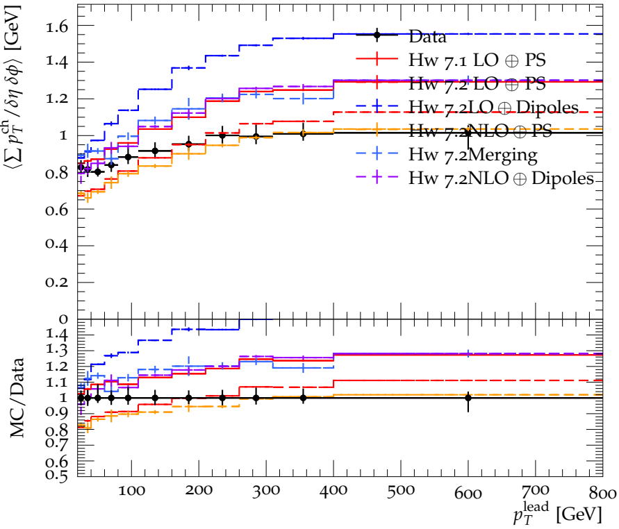
Trans-min \langle \sum p_T^{\text{ch}} / \delta\eta \delta\phi \rangle vs. p_T^{\text{lead}} in |\eta| < 2.5 in incl jet events
