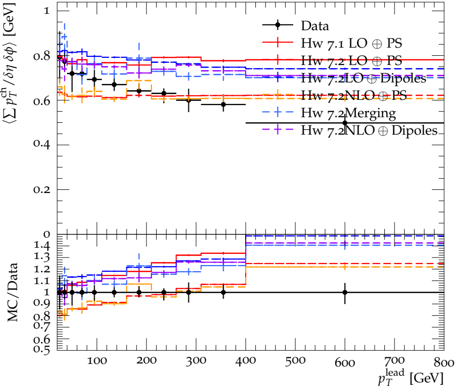
Trans-min \langle \sum p_T^{\text{ch}} / \delta\eta \delta\phi \rangle vs. p_T^{\text{lead}} in |\eta| < 2.5 in excl dijet events
