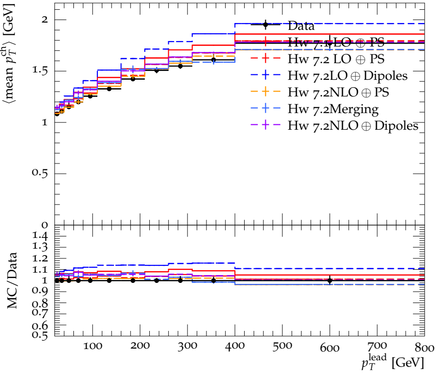
Transverse \langle \text{mean } p_T^{\text{ch}} \rangle vs. p_T^{\text{lead}} in |\eta| < 2.5 in incl jet events
