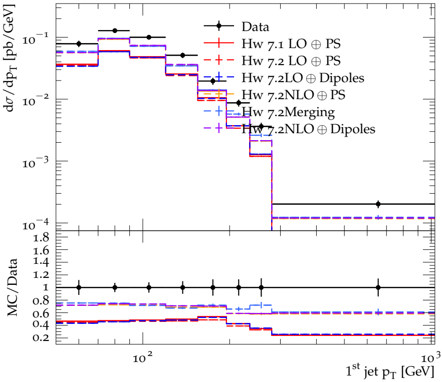
t\bar{t} cross-section vs. 1 st jet p_T
