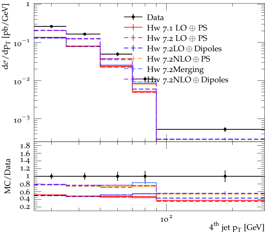
t\bar{t} cross-section vs. 4 th jet p_T
