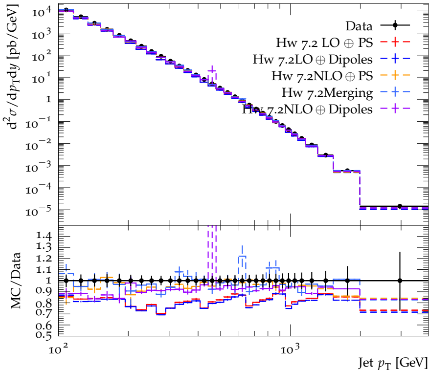
Inclusive jet cross section as a function of jet p_T ( 0.5 < |y| < 1.0 )
