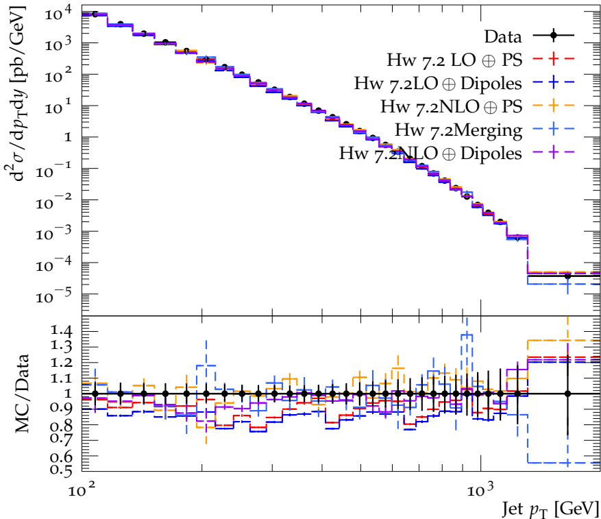
Inclusive jet cross section as a function of jet p_T ( 1.5 < |y| < 2.0 )
