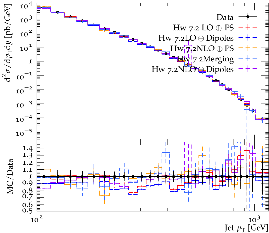
Inclusive jet cross section as a function of jet p_T ( 2.0 < |y| < 2.5 )
