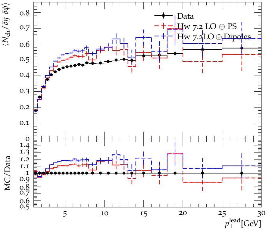
Mean charged-particle multiplicity density, trans-diff region
