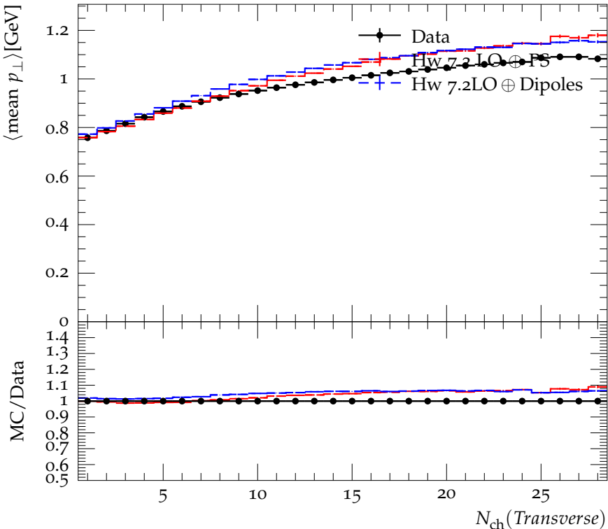
Mean average transverse momentum, transverse region
