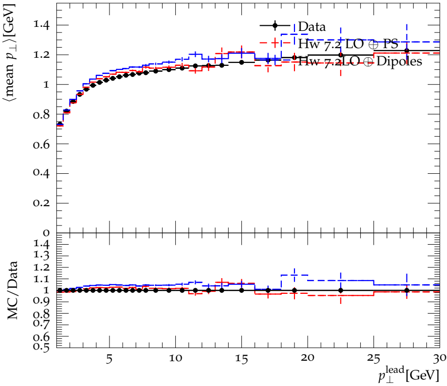
Mean average transverse momentum, transverse region
