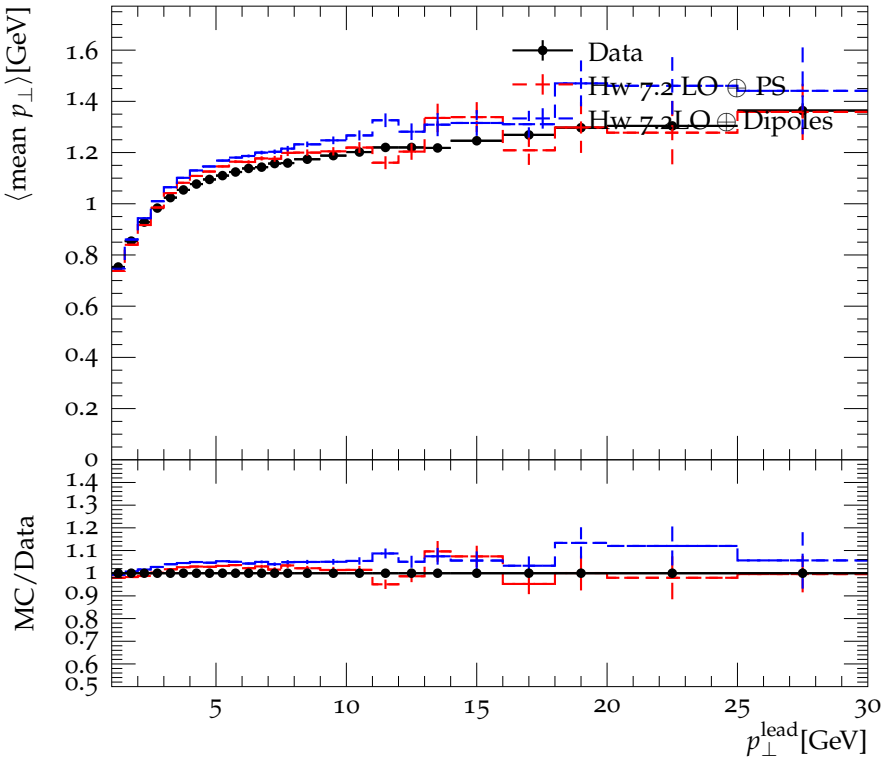
Mean average transverse momentum, trans-max region
