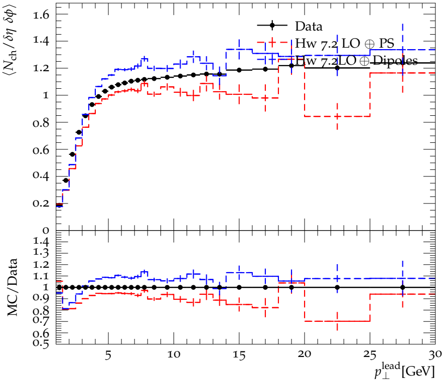
Mean charged-particle multiplicity density, transverse region
