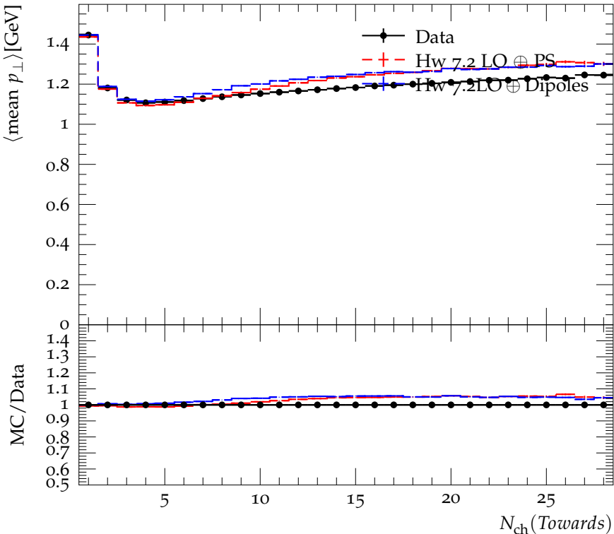
Mean average transverse momentum, towards region
