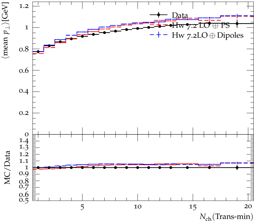
Mean average transverse momentum, trans-min region
