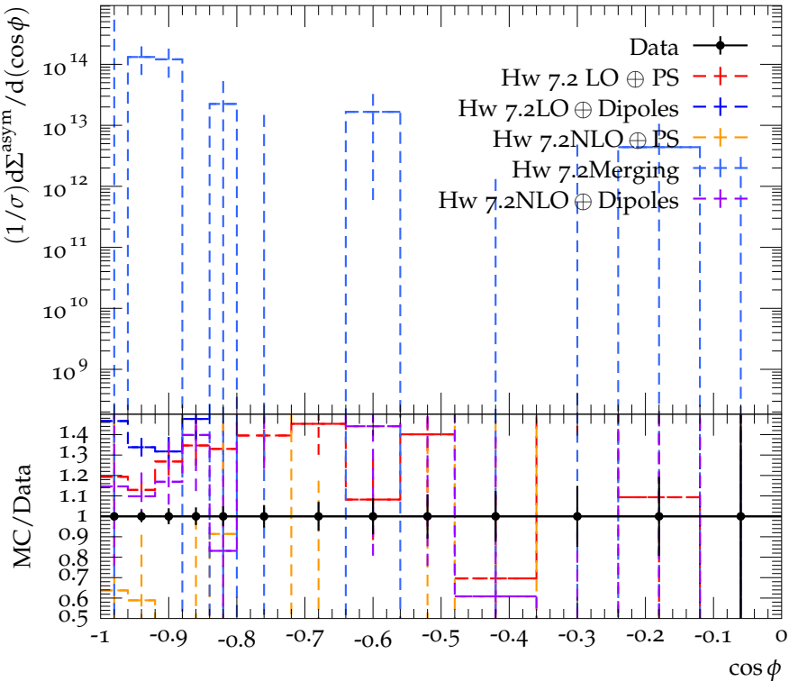
Transverse EEC asymmetry for 800 \text{ GeV} < H_{T2} < 850 \text{ GeV}
