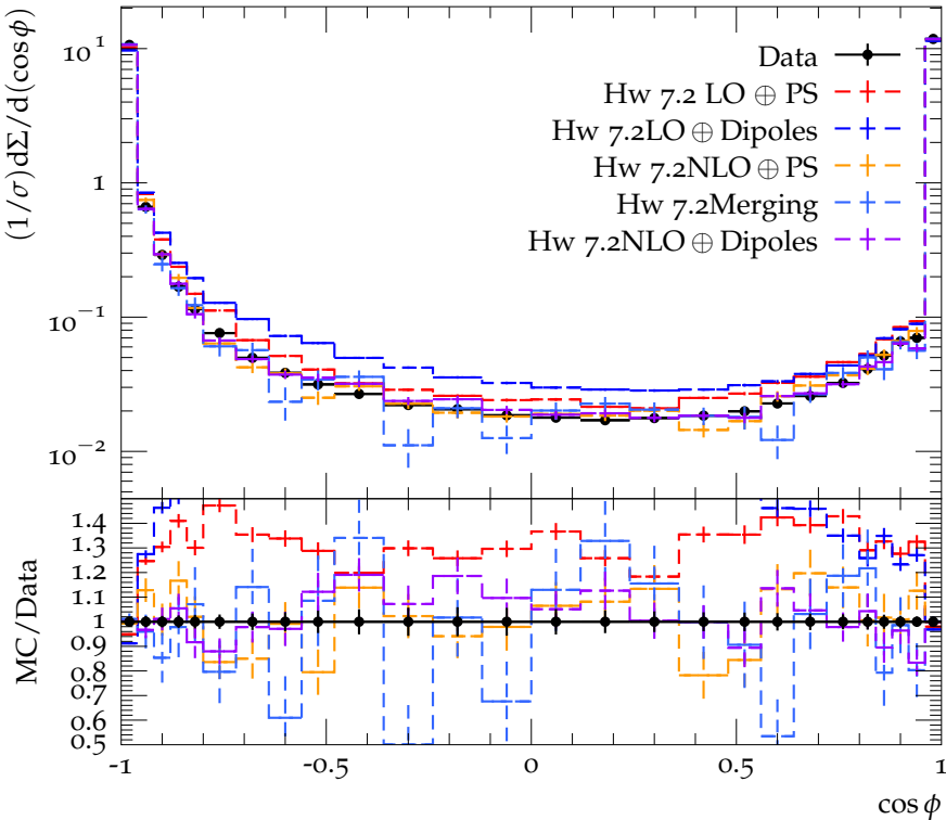
Transverse EEC for 900 \text{ GeV} < H_{T2} < 1000 \text{ GeV}
