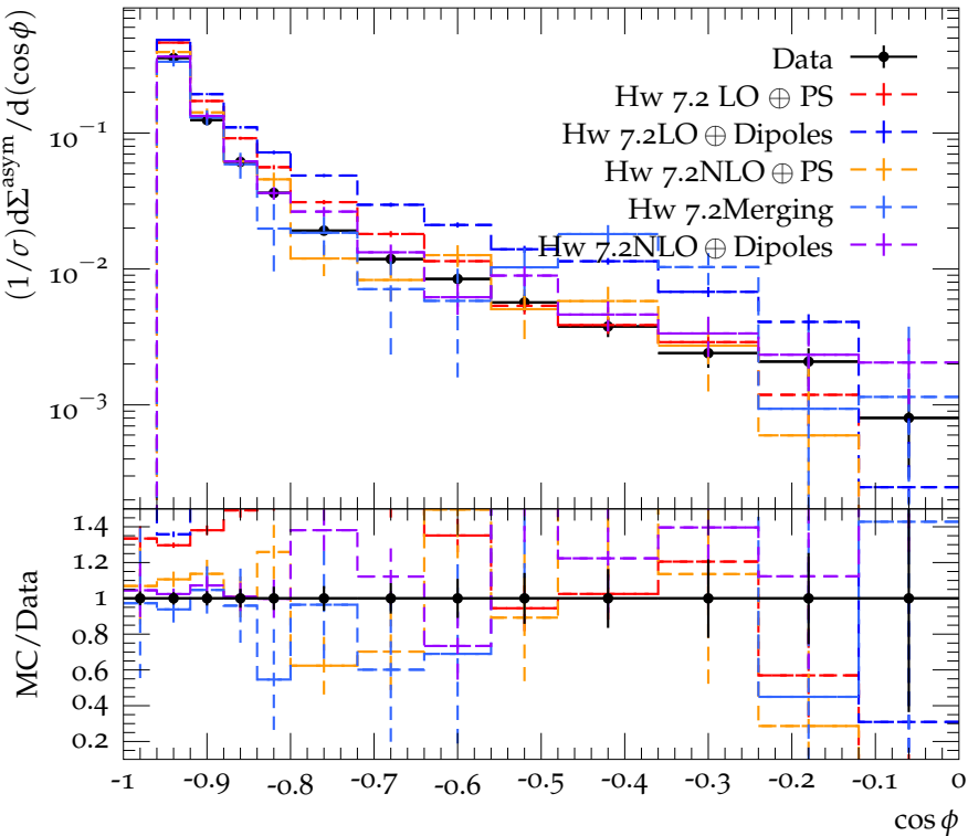
Transverse EEC asymmetry for H_{T2} > 1400 GeV
