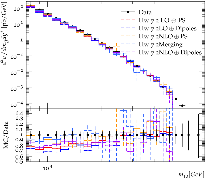
Dijet cross section ( 1.5 \leq y^* < 2.0 ), R=0.4
