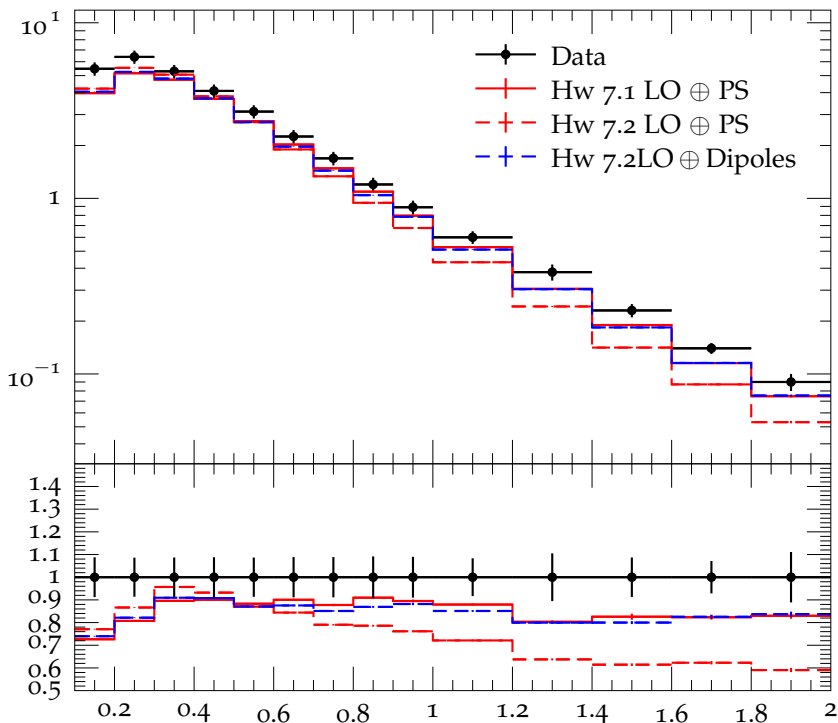
Charged hadron p_{\perp} for |\eta| = 0.3 at \sqrt{s} = 0.9 TeV
