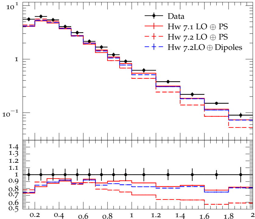
Charged hadron p_{\perp} for |\eta| = 0.5 at \sqrt{s} = 0.9 TeV
