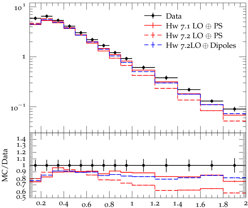
Charged hadron p_{\perp} for |\eta| = 0.9 at \sqrt{s} = 0.9 TeV
