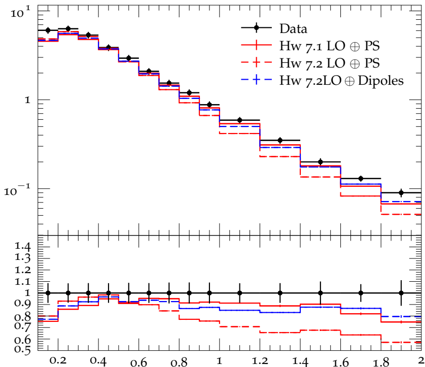
Charged hadron p_{\perp} for |\eta| = 1.1 at \sqrt{s} = 0.9 TeV
