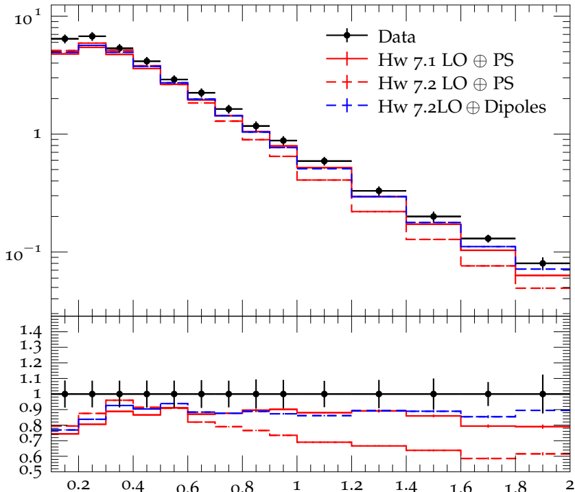
Charged hadron p_{\perp} for |\eta| = 1.5 at \sqrt{s} = 0.9 TeV
