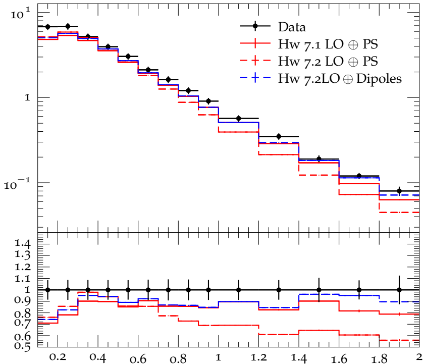
Charged hadron p_{\perp} for |\eta| = 1.7 at \sqrt{s} = 0.9 TeV
