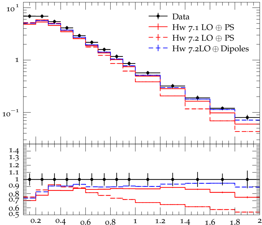
Charged hadron p_{\perp} for |\eta| = 1.9 at \sqrt{s} = 0.9 TeV
