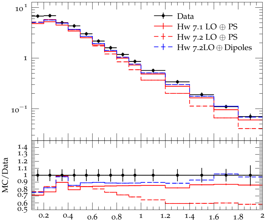
Charged hadron p_{\perp} for |\eta| = 2.1 at \sqrt{s} = 0.9 TeV
