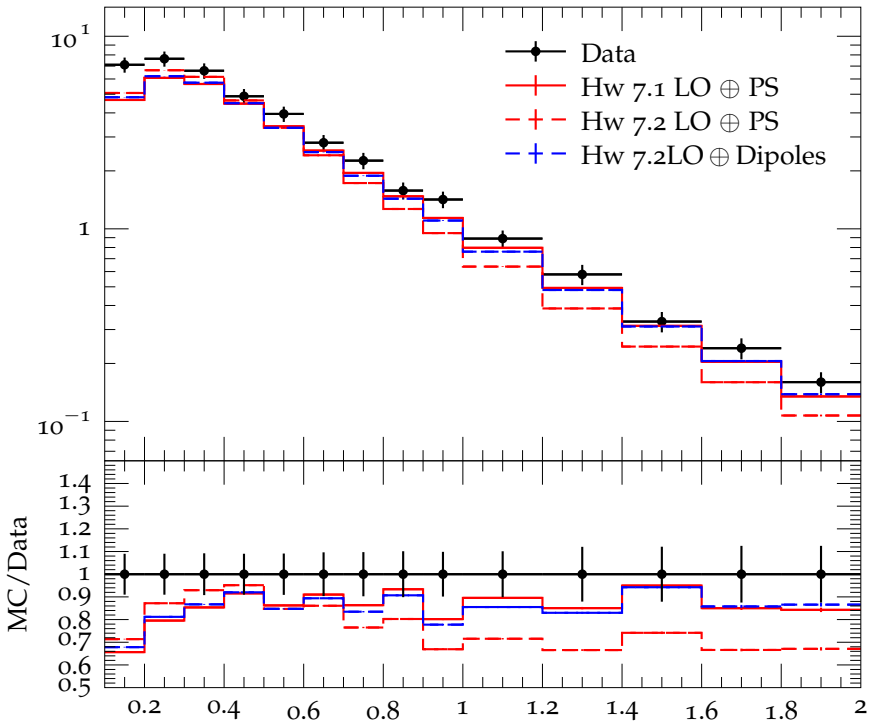
Charged hadron p_{\perp} for |\eta| = 0.3 at \sqrt{s} = 2.36 TeV
