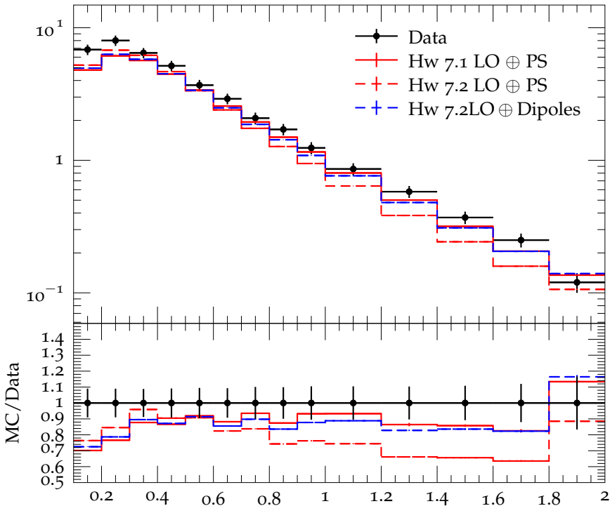
Charged hadron p_{\perp} for |\eta| = 0.5 at \sqrt{s} = 2.36 TeV
