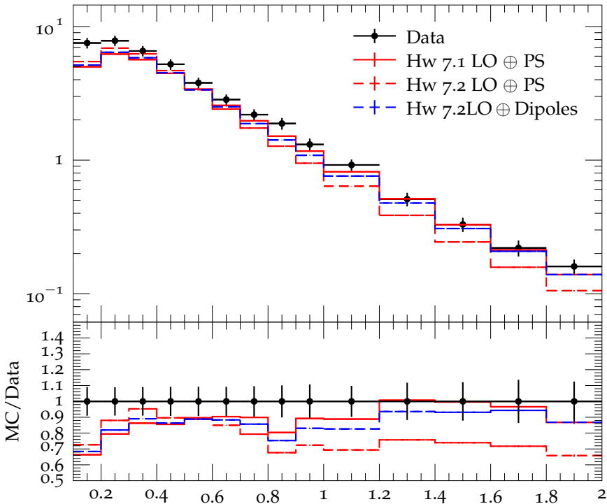
Charged hadron p_{\perp} for |\eta| = 0.7 at \sqrt{s} = 2.36 TeV
