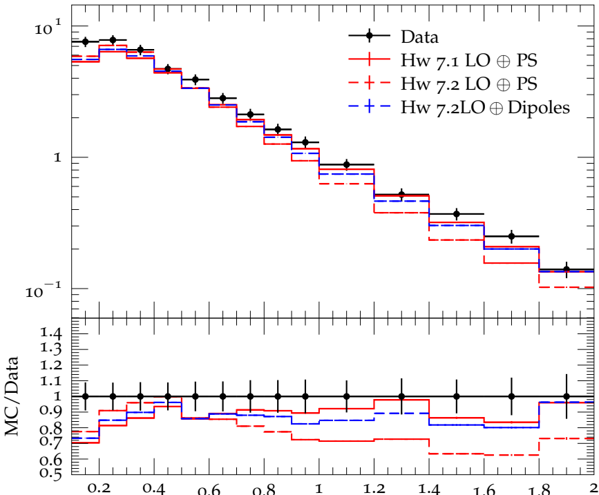
Charged hadron p_{\perp} for |\eta| = 1.1 at \sqrt{s} = 2.36 TeV
