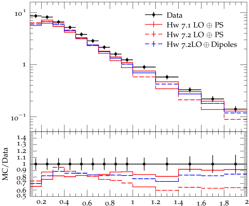
Charged hadron p_{\perp} for |\eta| = 1.9 at \sqrt{s} = 2.36 TeV
