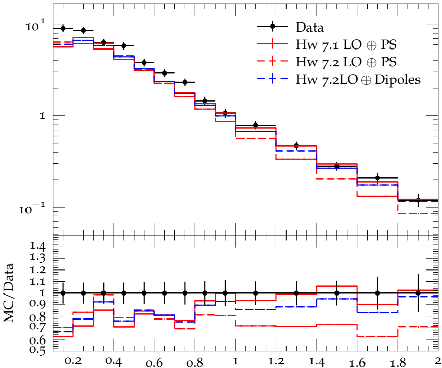
Charged hadron p_{\perp} for |\eta| = 2.1 at \sqrt{s} = 2.36 TeV
