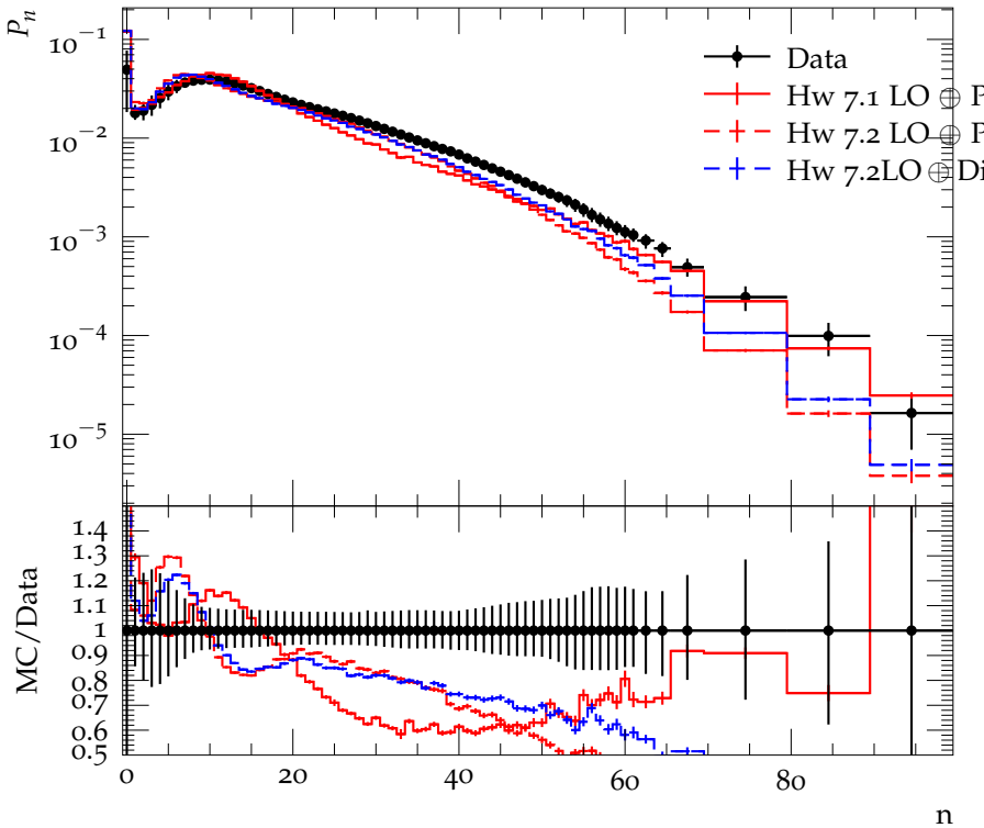
Charged hadron multiplicity, |\eta| < 2.4 , \sqrt{s} = 0.9 TeV
