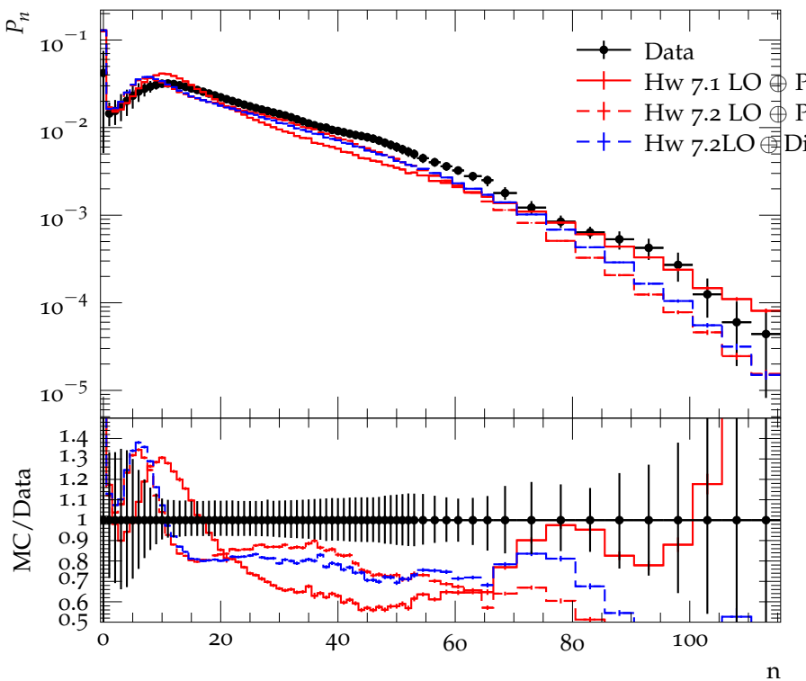
Charged hadron multiplicity, |\eta| < 2.4 , \sqrt{s} = 2.36 TeV
