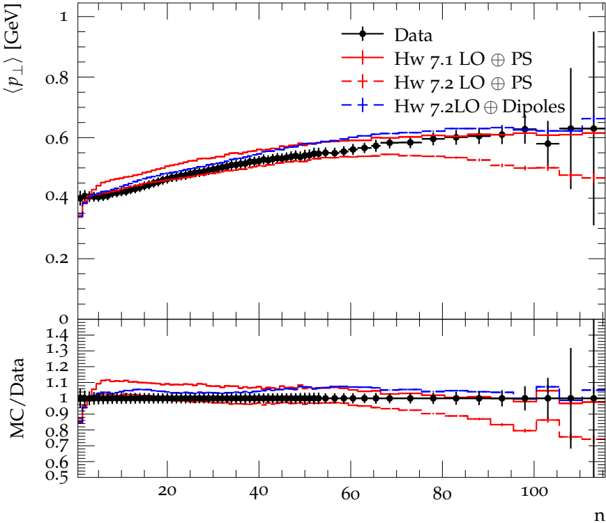
Mean p_{\perp} vs charged hadron multiplicity, |\eta| < 2.4 , \sqrt{s} = 2.36 TeV
