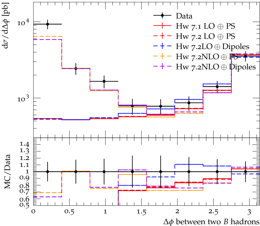
B\bar{B} production cross-section (leading jet p_{\perp} > 84 GeV)
