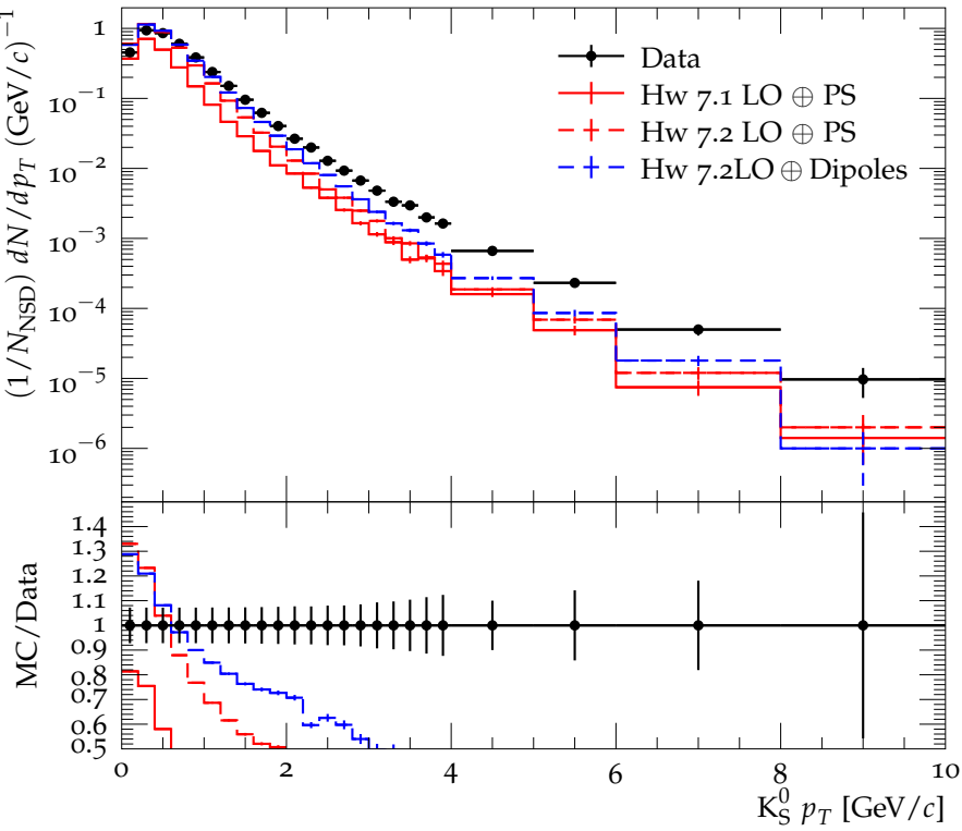
K_S^0 transverse momentum distribution at \sqrt{s} = 0.9 TeV
