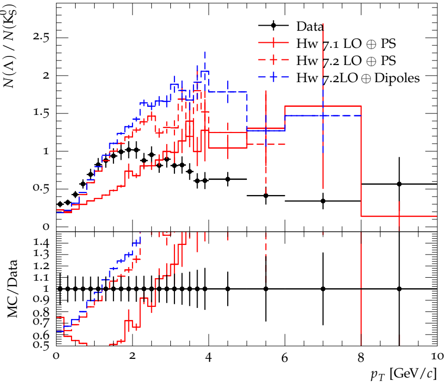
\Lambda/K_S^0 versus transverse momentum at \sqrt{s} = 0.9 TeV
