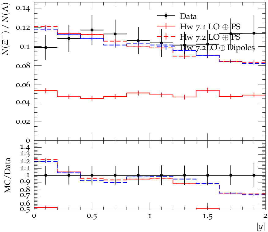
\Xi^- / \Lambda versus rapidity at \sqrt{s} = 0.9 TeV
