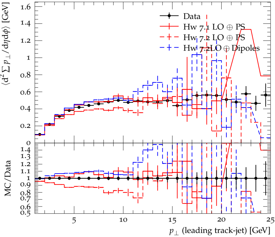
Transverse \Sigma p_{\perp} density vs. p_{\perp}^{\text{jet } 1} , \sqrt{s} = 900 GeV
